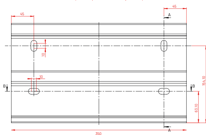
Support mural 350 mm
